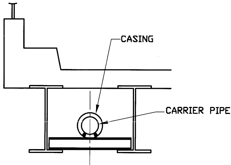
SECTION
