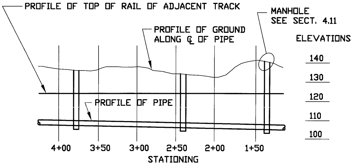
PROFILE - SEE SECT. 1.6 SCALE: HORIZ: _____ VERT: _____
