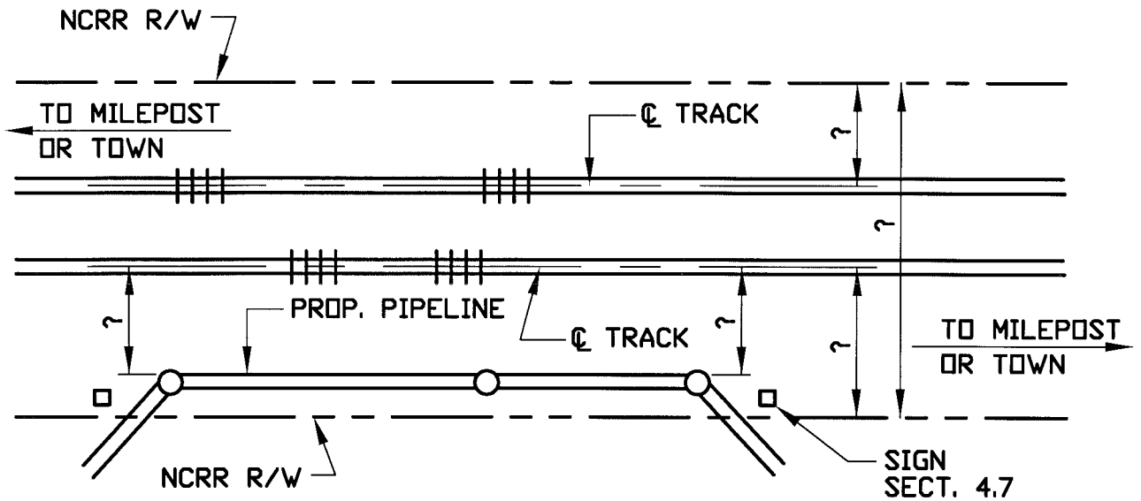
PLAN - SEE SECT. 1.6 SCALE OF DRAWING TO BE SHOWN
